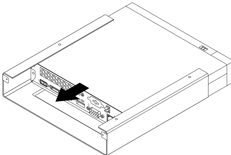
Figure 11. Installation du support de montage VESA
